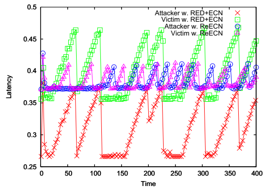
Fig. 15. RTT with DoS attack.
