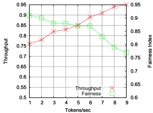
Fig. 5. Different tokens/sec.
