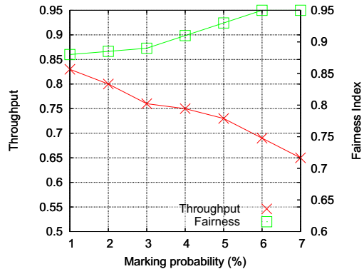
Fig. 6. Different marking probability.
