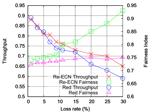
Fig. 8. Different congestion level.
