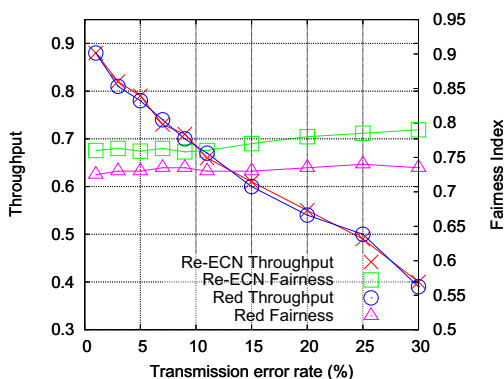
Fig. 13. Different transmission error rate (Infrastructure-model).
