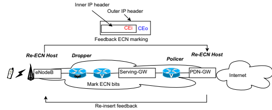
Fig. 3. Infrastructure based Re-ECN framework
