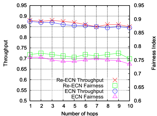
Fig. 10. Different hop count.
