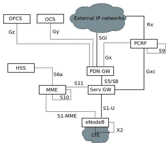
Fig. 1. LTE Architecture
